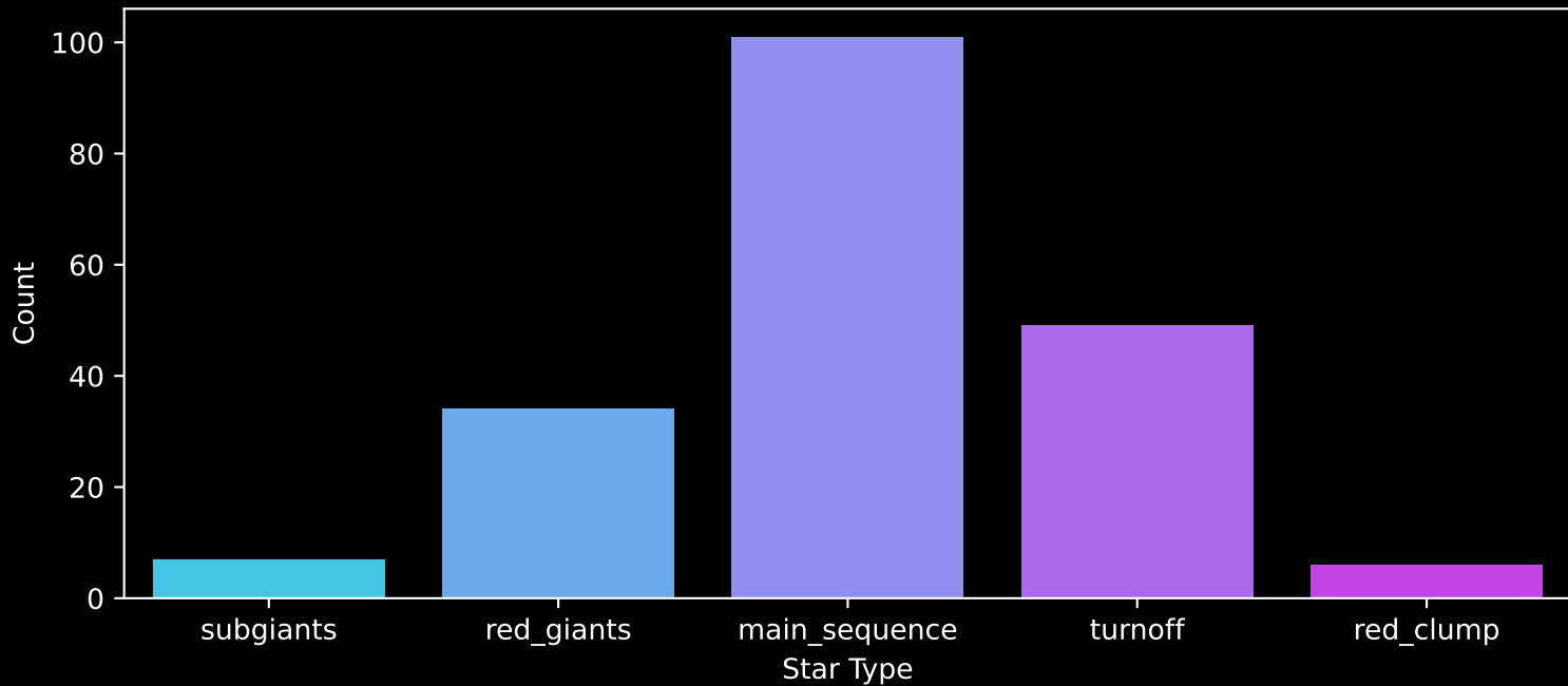
APOGEE DR17 Field: [141-47_MGA] Count plot of Star Type
