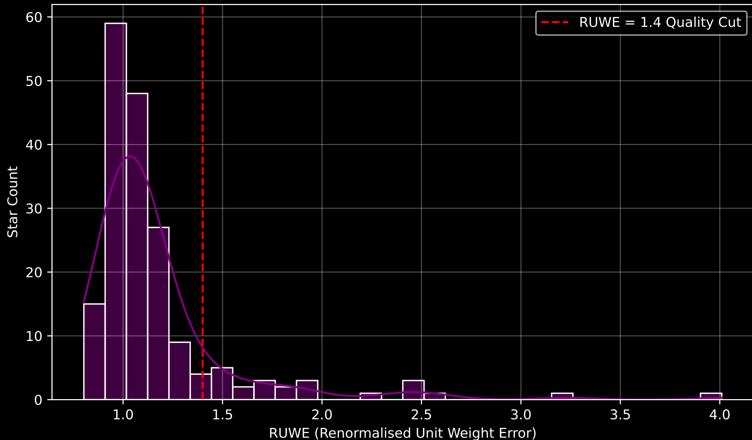
GAPOGEE DR17 Field [141-47_MGA] RUWE Distribution (n= 184)
