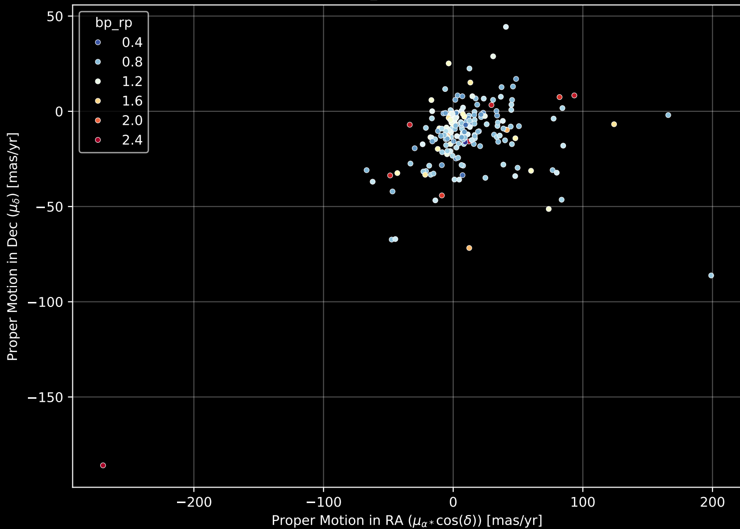
APOGEE DR17 Field: [141-47_MGA] Proper Motion Diagram (n= 197)
