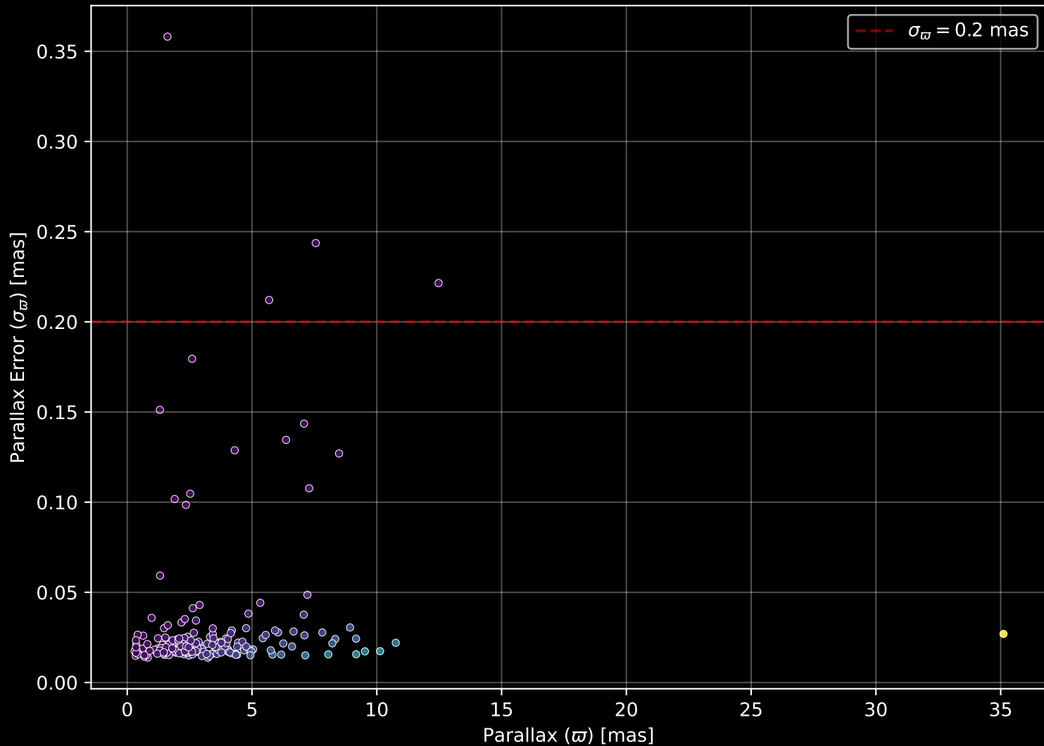
APOGEE DR17 Field: [141-47_MGA] Parallax Quality (n= 197)
