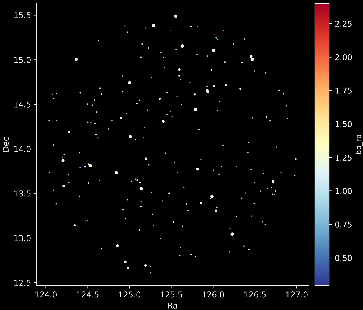
APOGEE DR17 Field: [141-47_MGA] Stars: 197
