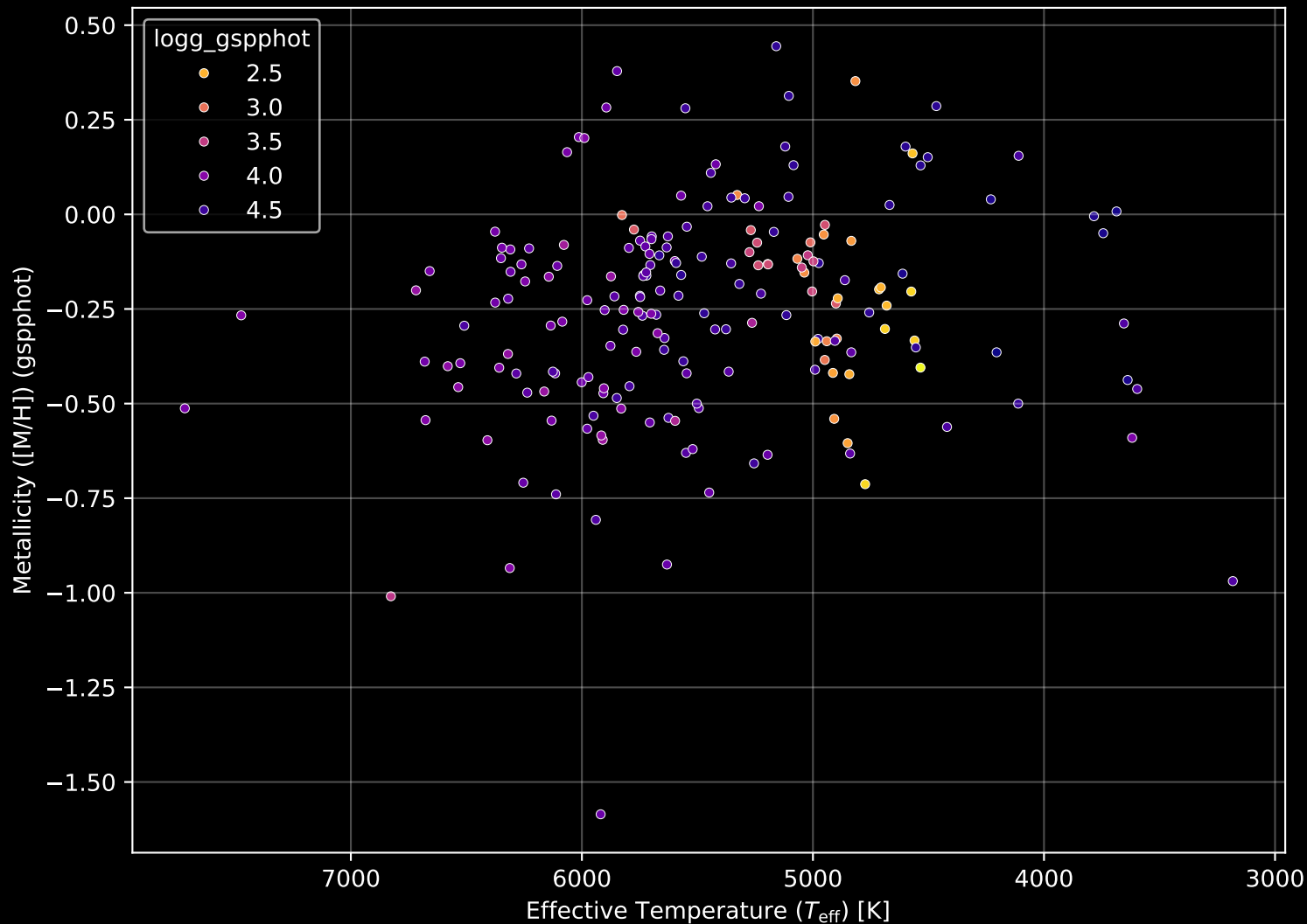
APOGEE DR17 Field: [141-47_MGA] Stellar Population Parameters (n= 197)
