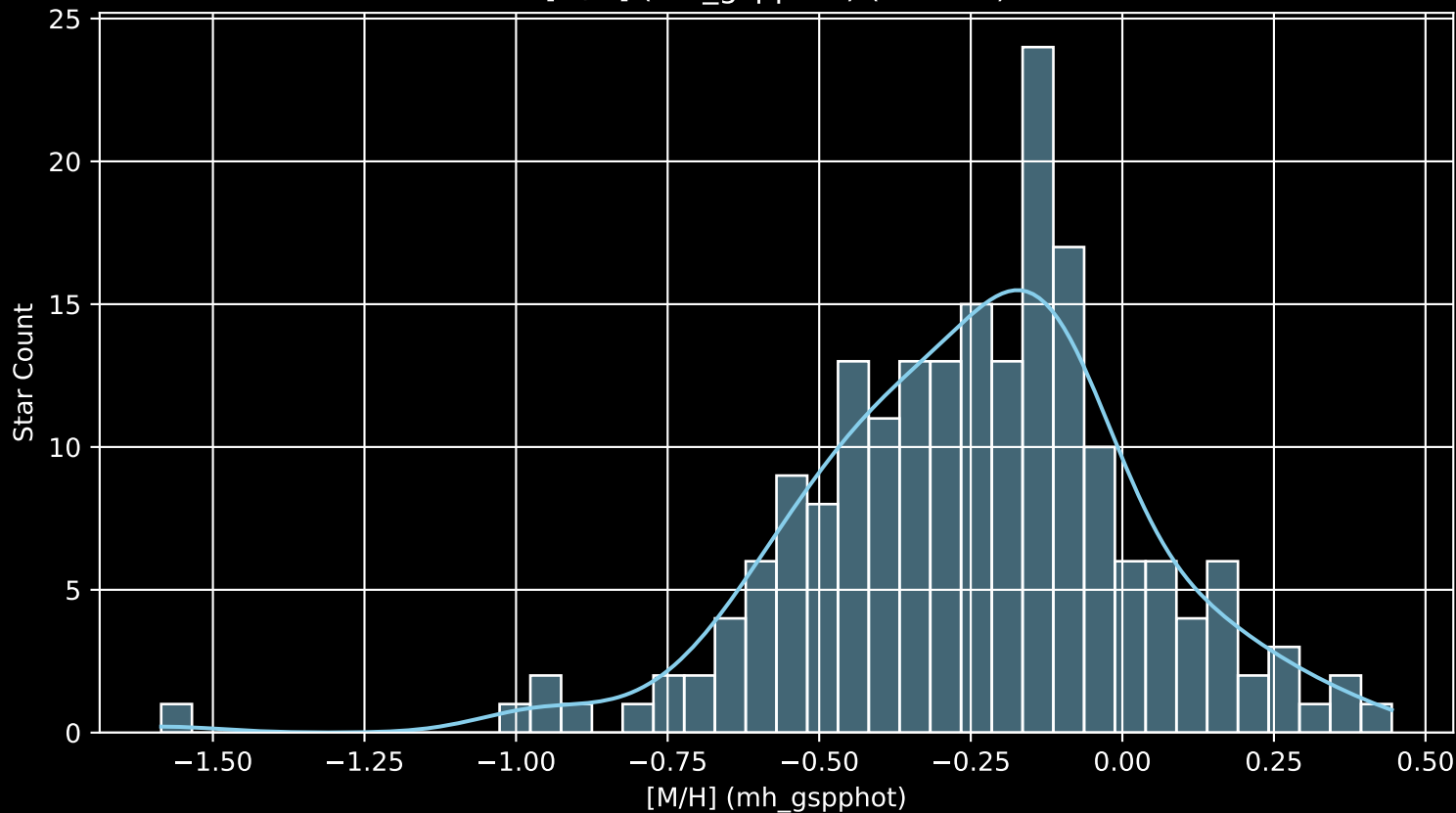
APOGEE DR17 Field: [141-47_MGA [M/H] (mh_gspphot) (n = 197)
